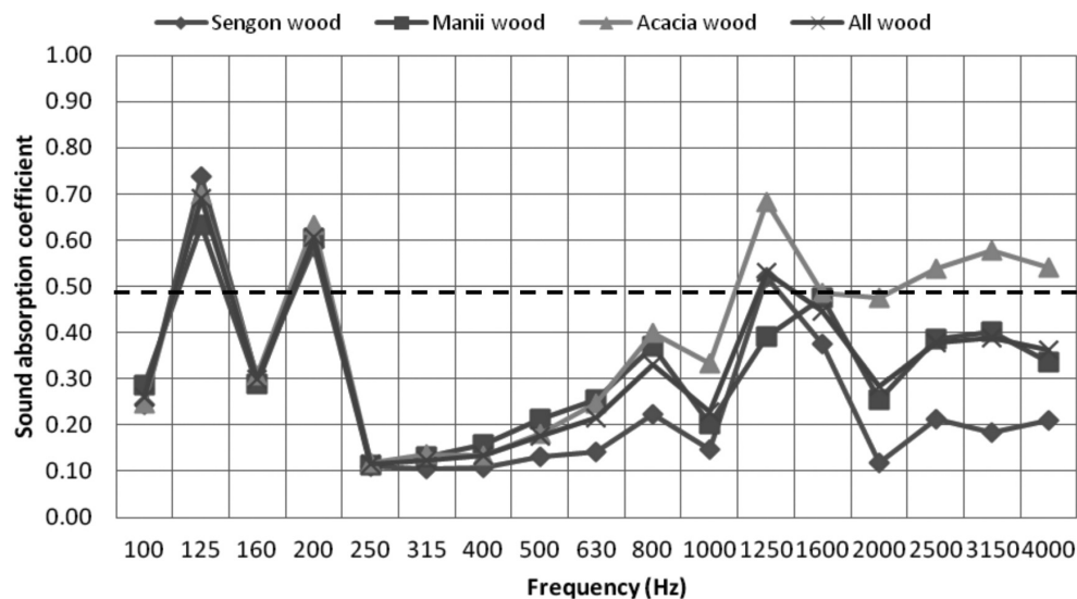
Figure 3 Sound absorption coefficient at different frequencies for medium-density particleboard (0.8 g cm -3 )
