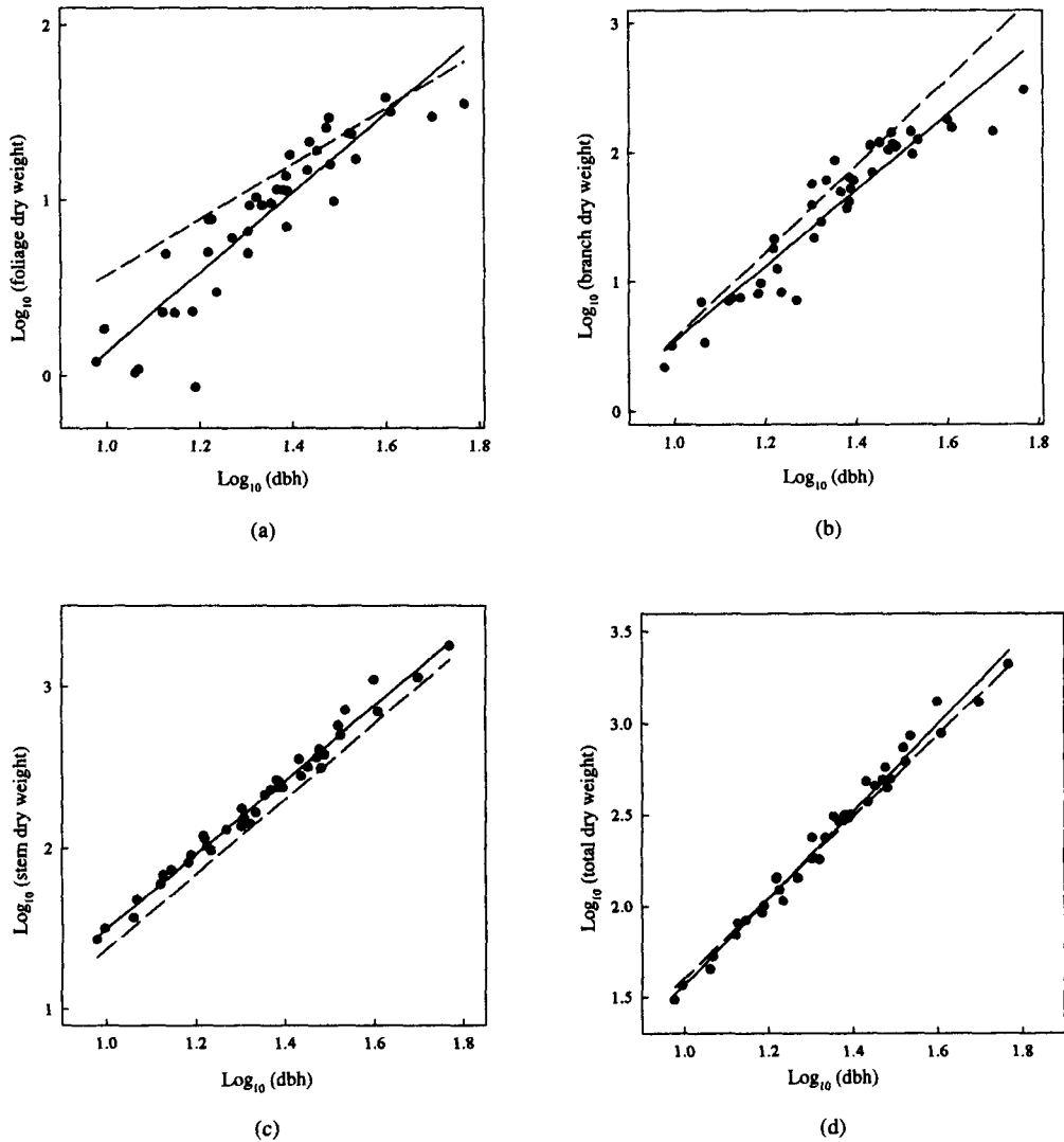
Figure 3 Comparison of allometric models developed in this study (continuous line) vs allometric models developed by Negi et al. (1995) (dashed line) for the relationships between (a) foliage dry weight, (b) branch dry weight, (c) stem dry weight and (d) total aboveground dry weight and dbh in Tectona grandis plantations in Costa Rica and in India respectively. Dots correspond to sample data of this study.
